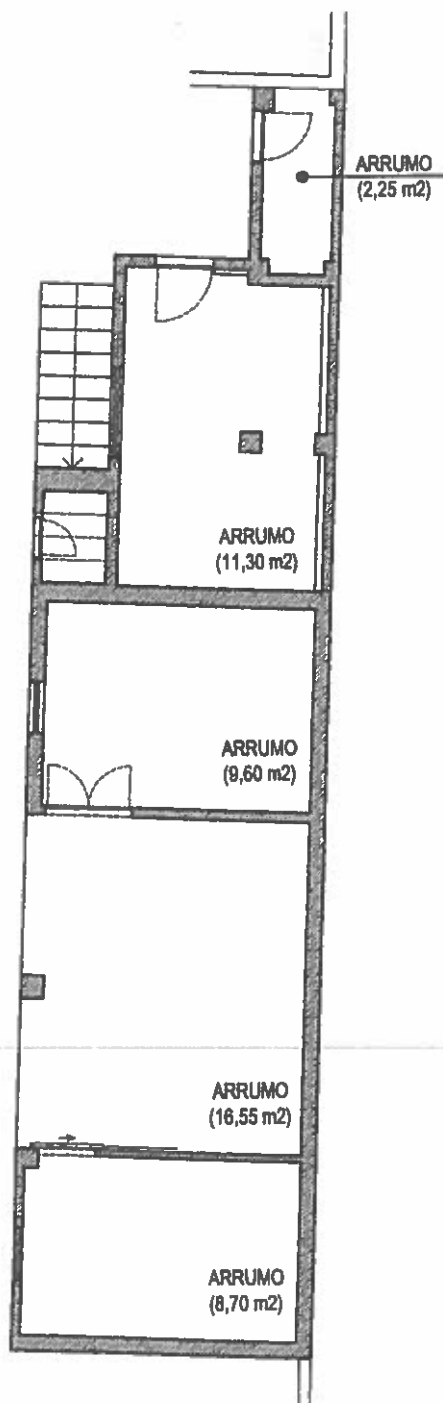
PLANTA DO R/CHÃO (a.b. 59,70m 2 )
